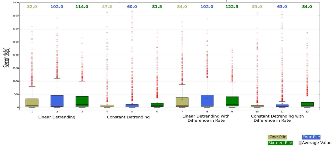
Figure 6.27: Comparison of change point detection methods for pheromone only parameters for P. rugosus . The time in seconds represents the difference between a pheromone laying event followed by a detection of change point in the foraging rate.
