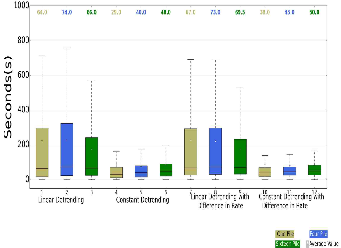
Figure 4.7: Comparison of change point detection methods without outliers for pheromone plus sitefidelity parameters . The time in seconds represents the difference between a pheromone laying event followed by a detection of change point in the foraging rate.
