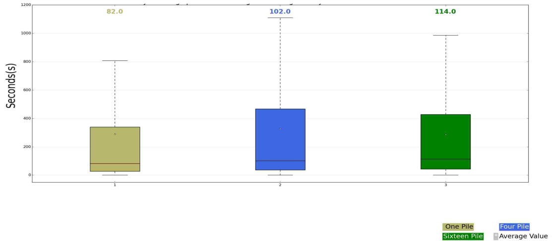
Figure 6.29: Efficiency of Linear Detrending method on data of P. rugosus for pheromone only settings
